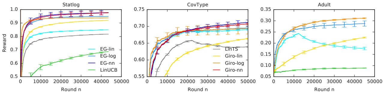
Figure 2. Comparison of Giro to LinUCB, LinTS, and the \epsilon -greedy policy on three contextual problems in Section 6.2. The reward is reported as a function of round n . The results are averaged over 5 runs. To reduce clutter, the legend is split between the first two plots.
